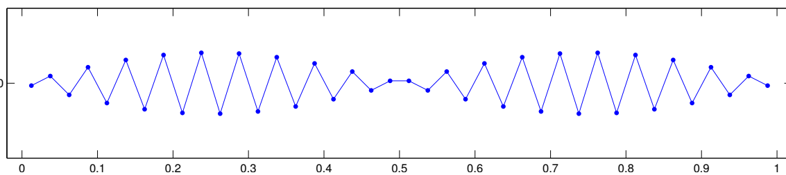
Figure 3.11. Nullspace of computed \frac{\partial f(x)}{\partial x}
